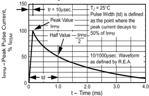
Fig. 3 – Pulse Waveform
